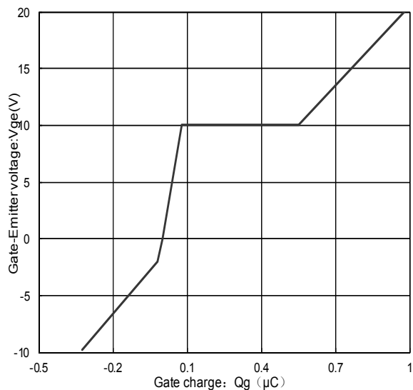
Dynamic Gate Charge(type)
